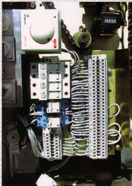
Control circuit of FPS op.mechanism
